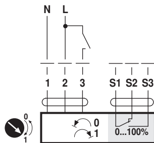
AC 230 V, open/close
